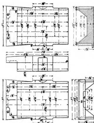
Figs. 4834-4838. Standard Wedge for Journal, 4\frac{1}{4} in. x 8 in. Plate 7.
